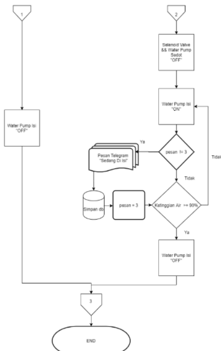
Gambar 2.4. flowchart 2
