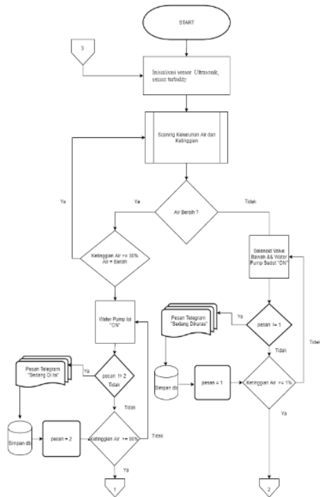
Gambar 2.3. flowchart 1
