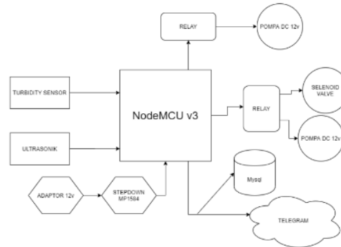
Gambar 2.2. Blok Diagram
