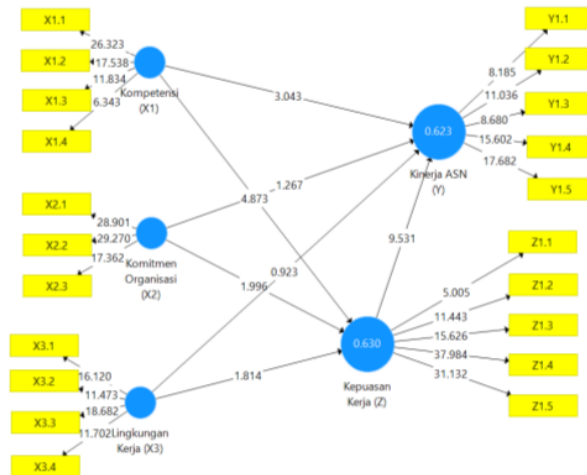
Gambar 5.5 Algorithm Bootstrapping report
