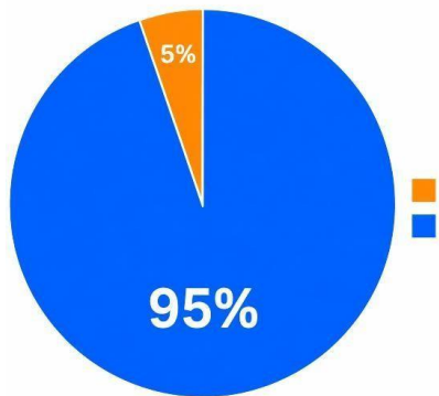
Gambar 4. 1 Hasil Uji Normalitas Data Model P-Plot
