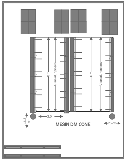
Picture 9. Winding Layout Before Improvement
