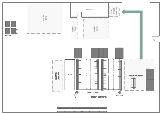
Picture 12. Packing Layout After Improvement
