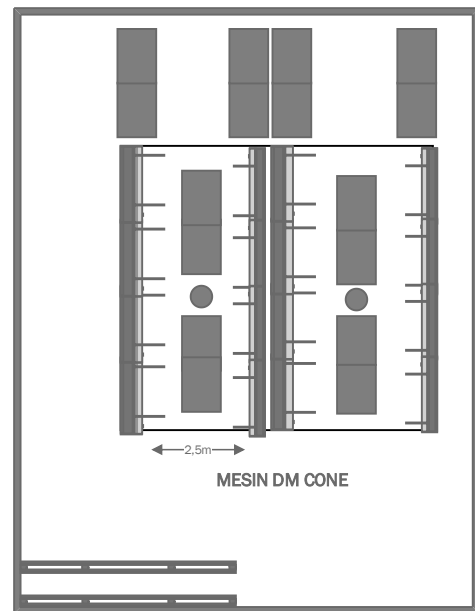
Picture 10. Winding Layout Before Improvement
