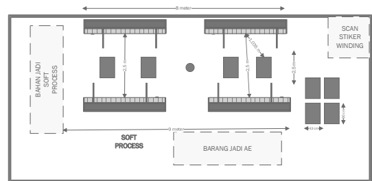
Picture 8. Layout Soft Process After Improvement
