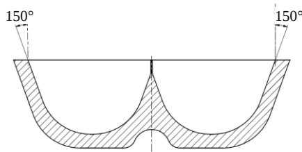
Figure 6. Bucket Design 150°
