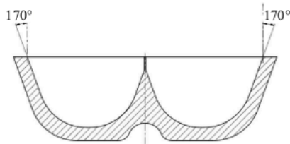
Figure 8. Bucket Design 170°
