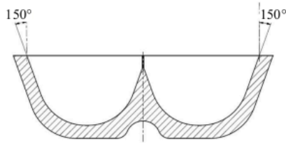
Figure 6. Bucket Design 150°
