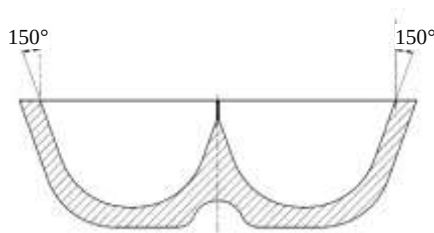
Figure 6. Bucket Design 150°
