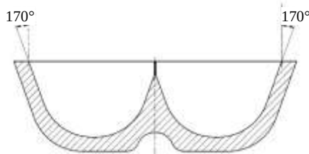
Figure 8. Bucket Design 170°
