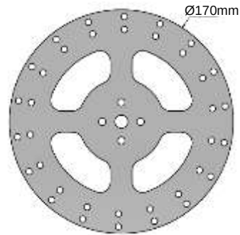
Figure 2. Runner Diameter 170 mm
