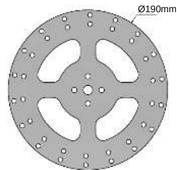
Figure 3. Runner Diameter 190 mm
