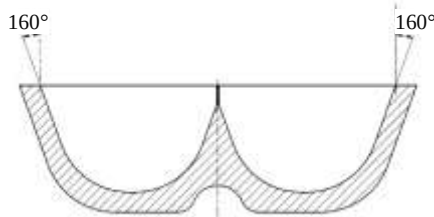
Figure 7. Bucket Design 160°
