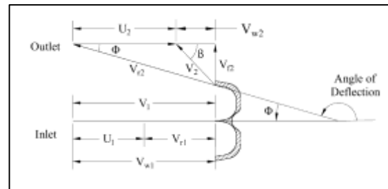
Figure 10. Pelton Turbine Velocity Triangle Cycle
