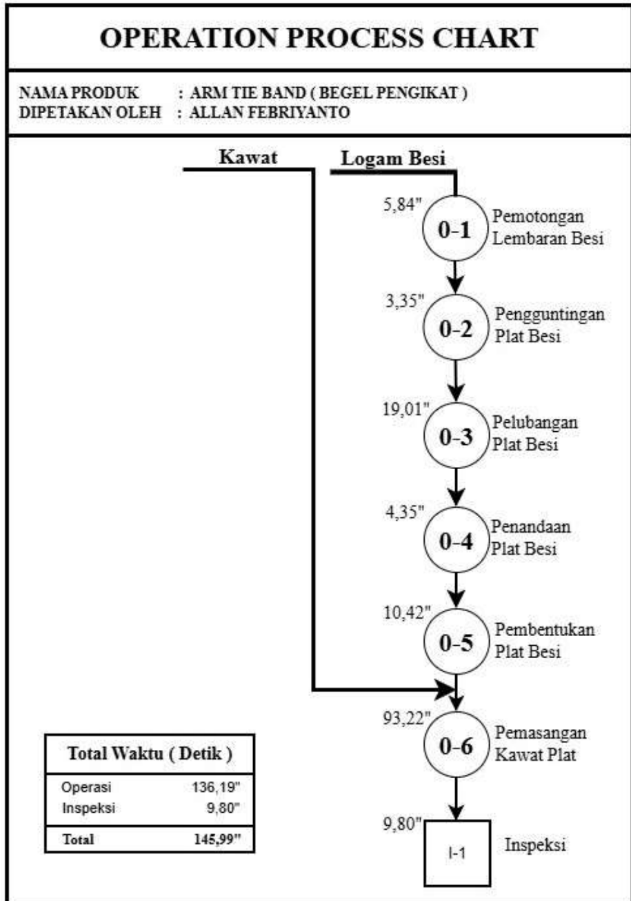
Lampiran 1. Operation Process Chart Produk Arm tie band
