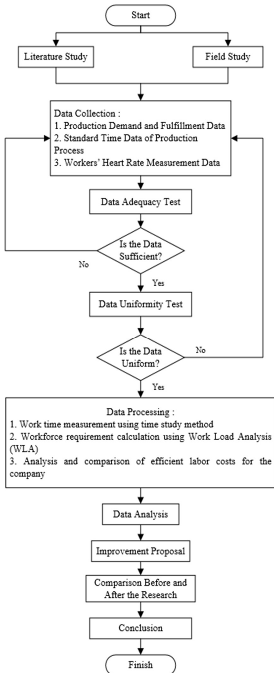
Figure 1 Research Flowchart
