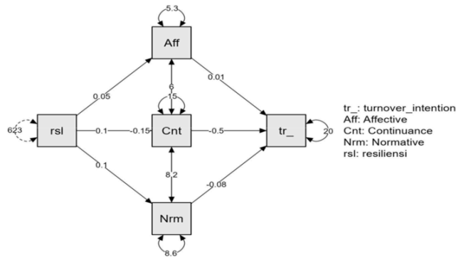
Figure 2. Path Analysis
