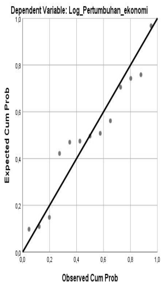
Normal P-P Plot of Regression Standardized Residual
