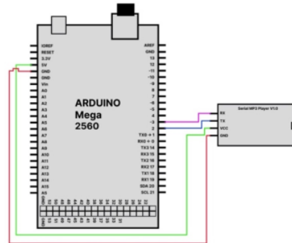
Gambar. 6 Serial Mp3 Player
