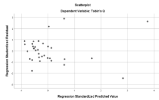
Gambar 4. Hasil Heteroscedasticity Test
