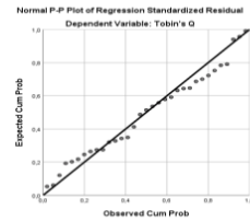
Gambar 2. Hasil Normality Test
