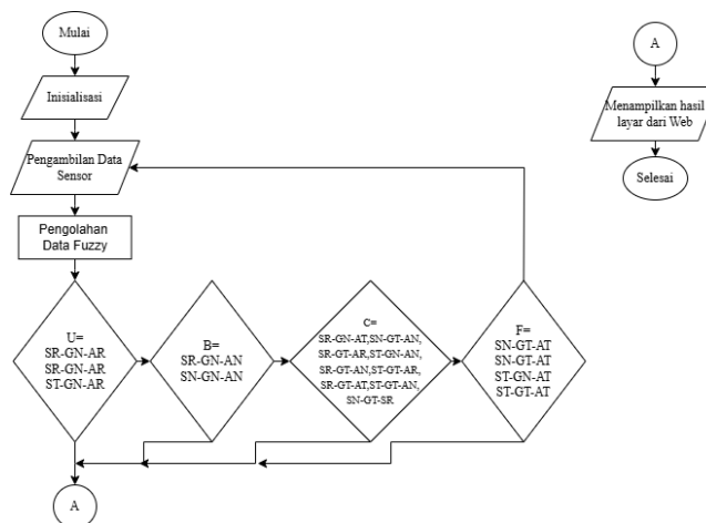
Gambar 3. Flowchart Sistem
