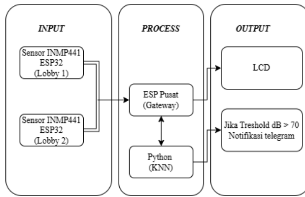
Gambar 2. Blok Diagram
