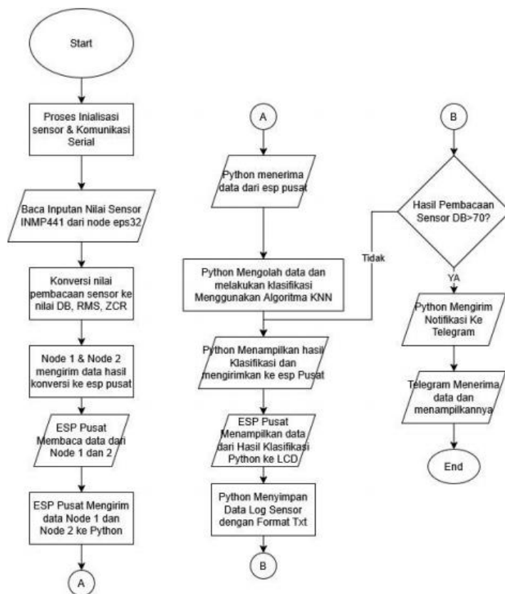
Gambar 1. Flowchart System
