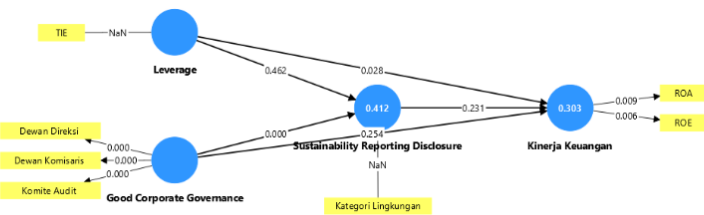
Gambar 7. Diagram SEM hasil bootstrapping
