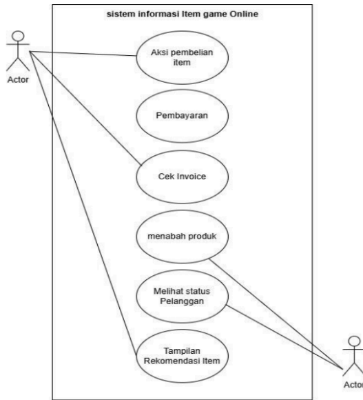
Gambar 1. Use Case Diagram Item Game
