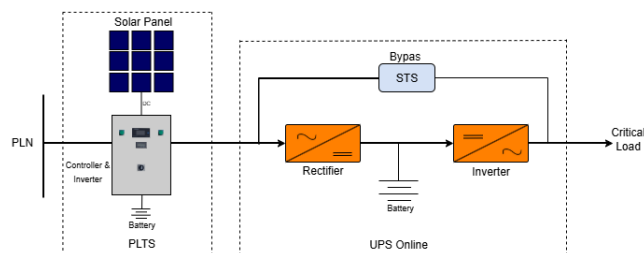
figure 2. 3 UPS Online
