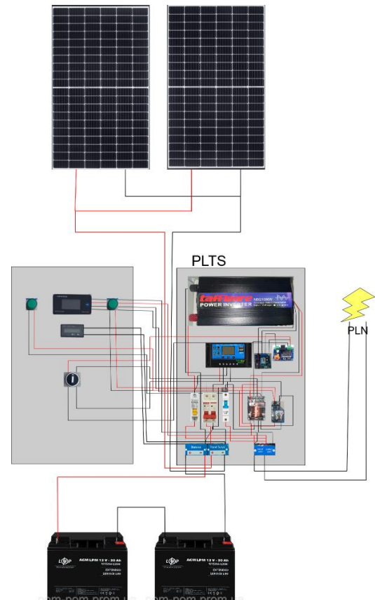
figure 2. 2 PLTS
