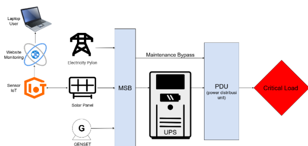
figure 2. 1 Desain Sistem Hybrid
