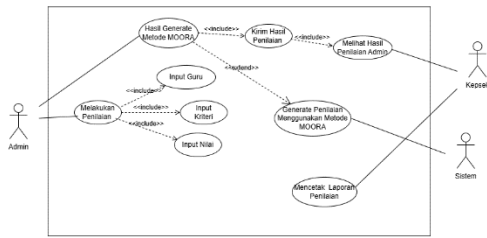
Gambar 3. Use Case Diagram
