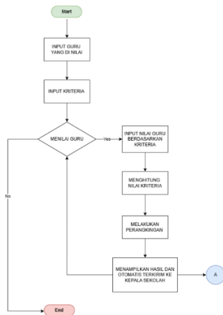
Gambar 4. User Flow Admin
