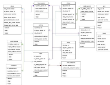
Gambar 4. Class Diagram
