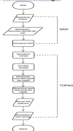
Gambar 5. Flowchart Perhitungan
