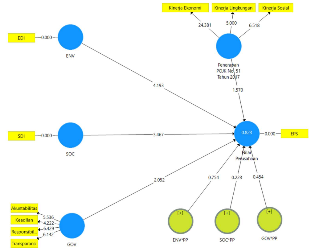
Path Coefficients
