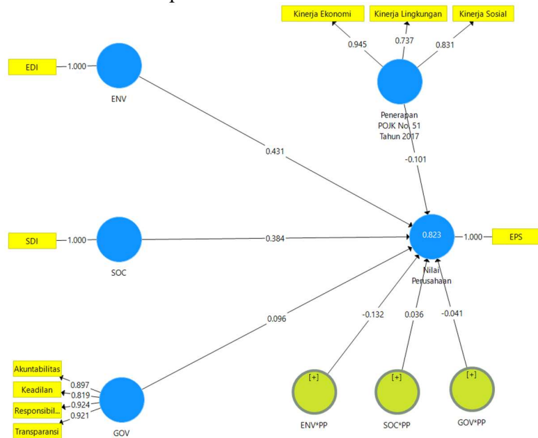
Outer Loadings
