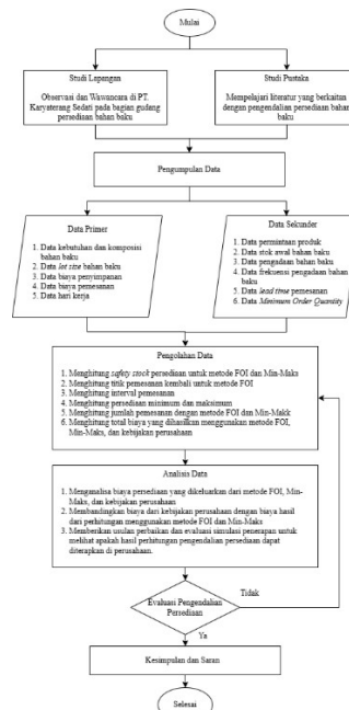
Gambar 1. Flowchart penelitian
