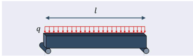
Gambar 3 Tegangan Bending
