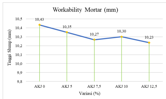
Gambar 3. Grafik Workability Mortar
