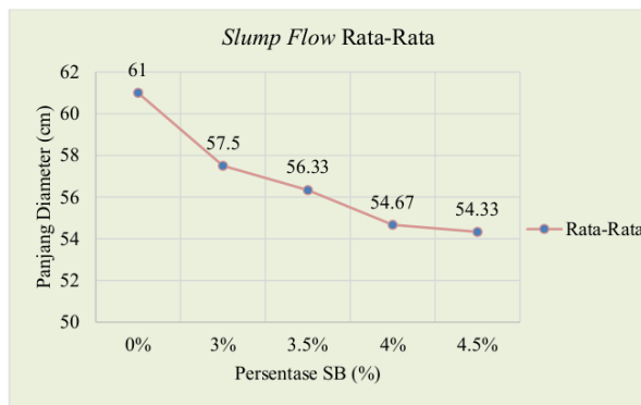
Gambar 5 Grafik Rata-Rata Slump Flow
