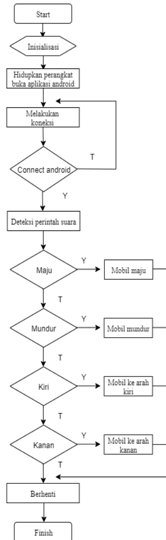
Gambar 2. Flowhart Sistem
