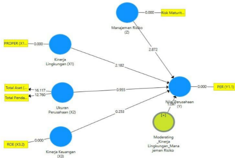
Gambar 2 Hasil Bootstrapping
