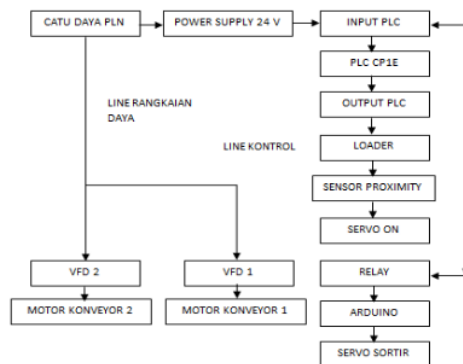
Gambar 1. Diagram Blok Sistem Kendali
