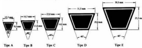
Gambar 2.2 V-Belt Konvensional Tipe Standard
