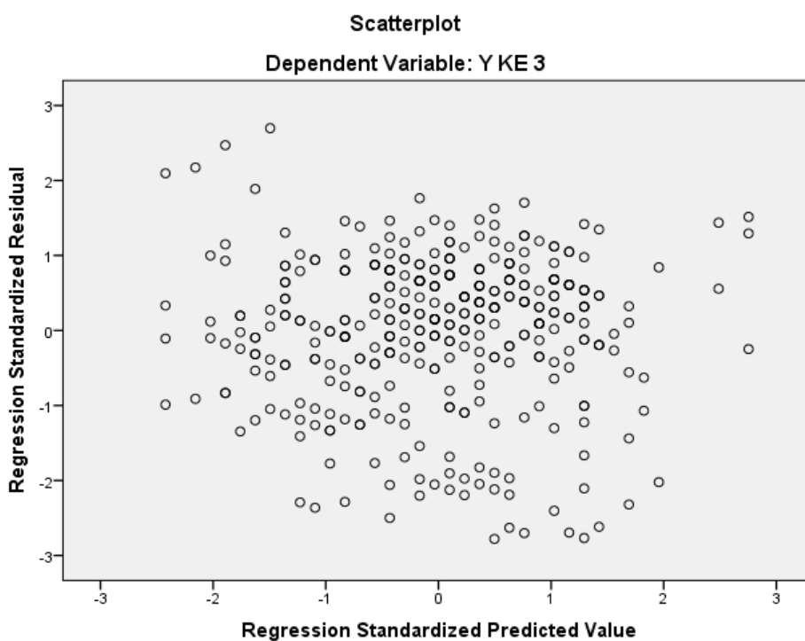
Gambar 2 Tampilan Scatterplot
