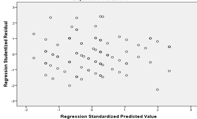
Scatterplot
