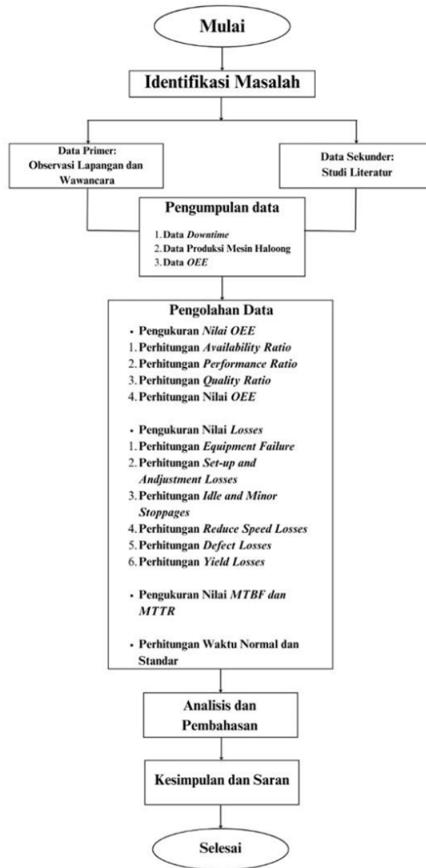
Gambar 2 Flowchart Penelitian
