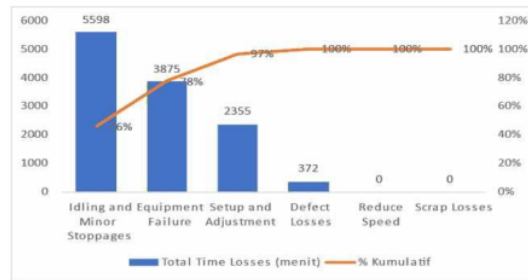
Gambar 3 Diagram Pareto Analisis Six Big Losses
