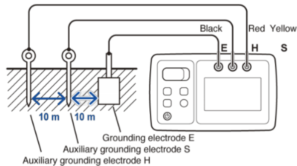
7 Figure 2. Soil Resistivity Measurement Circuit Using the Three Electrode Method
