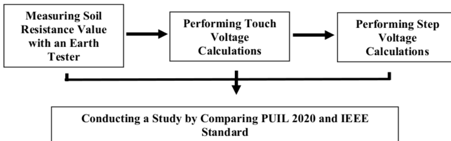
Figure 1. Block Diagram for the Process of Conducting a Study at Haji Regional Hospital
