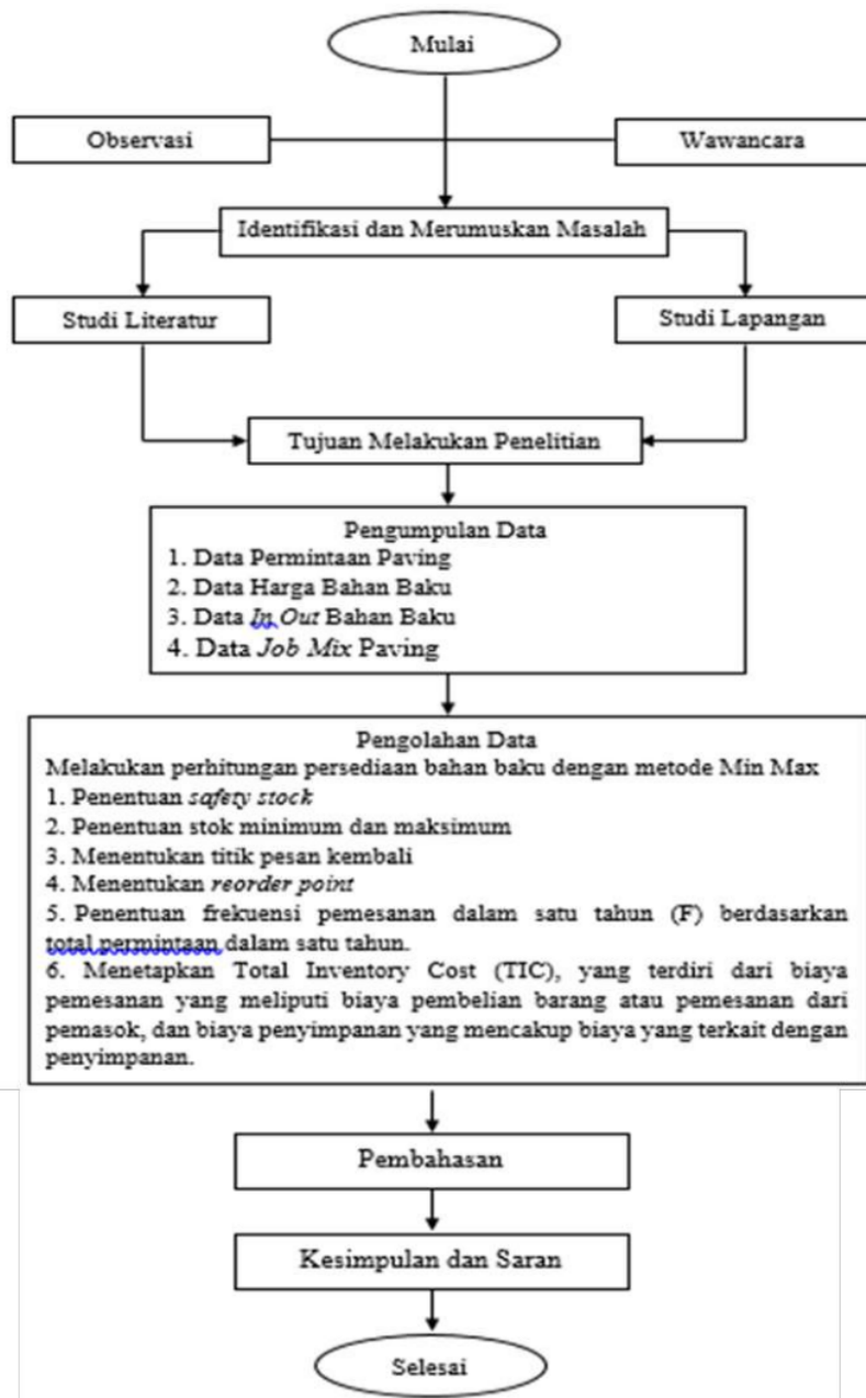
Gambar 1 Flowchart Penelitian
