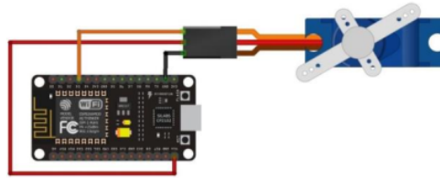
Figure 7. Rangkaian Servo
