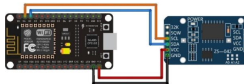
Figure 6. Rangkaian RTC
