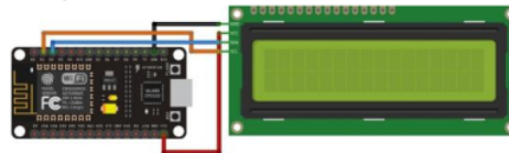
Figure 4. Rangkaian LCD 16x2 i2c
