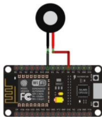
Figure 8. Rangkaian Buzzer
