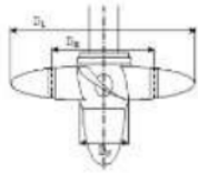
Gambar 9. Sketsa Gambar Diameter Turbin Kaplan
