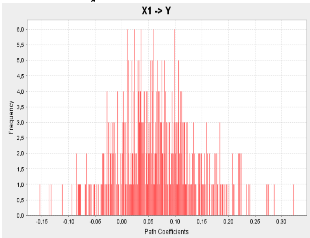
Path Coefficients Histogram
