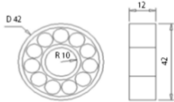
Gambar 7. Bearing NTN 6004LLU
