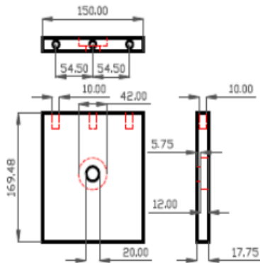
Gambar 11. Desain Tiang Penahan II
