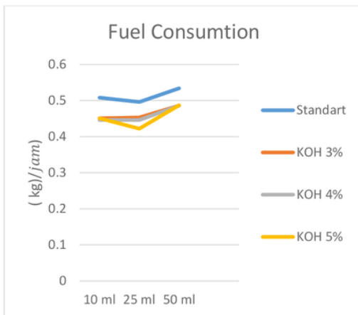
Grafik 4. Fuel Consumption
