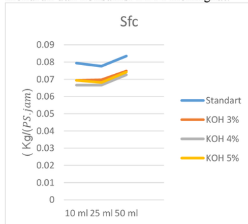
Grafik 5. Spesific Fuel Consumption
