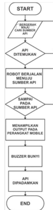
Gambar 2.2 Flowchart
