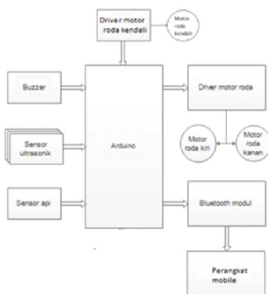
Gambar 2.1 Block Diagram
