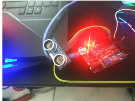
Gambar 3.4 Sensor Ultrasonik
