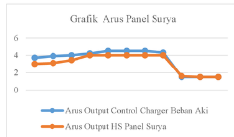
Gambar 4.3 Grafik arus Panel Surya
