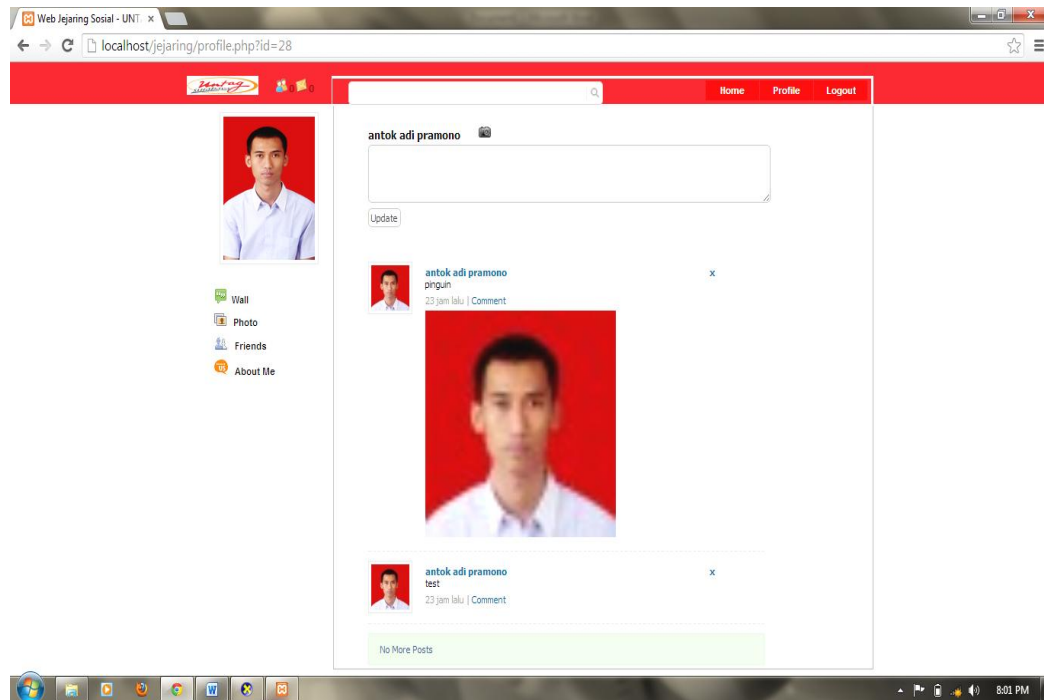
Gambar 4.5 Tampilan Profile
