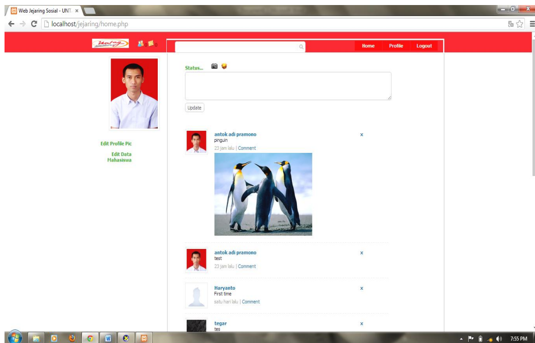
Gambar 4.4 Tampilan home
