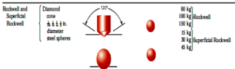
Gambar 12. Indentor pengujian rockwell (Callister, 2007)
