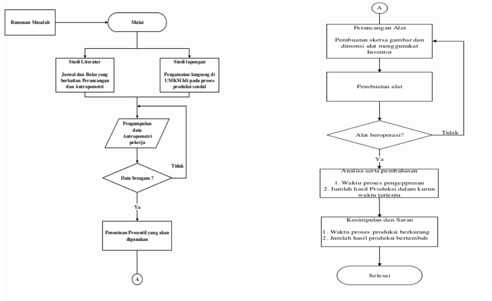
Gambar 3. Flowchart Penelitian
