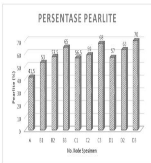
Gambar 11. Diagram Nilai Persentase Pearlite
