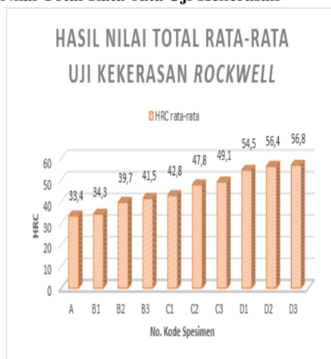
Gambar 9. Diagram Nilai Rata-rata Uji Kekerasan
