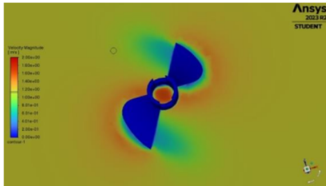
Gambar 6. Contour Velocity FPP ø40 2 pitch
