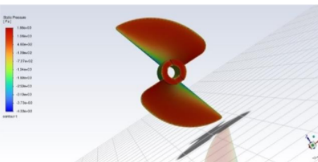
Gambar 11. Contour Pressure FPP ø70 2 pitch
