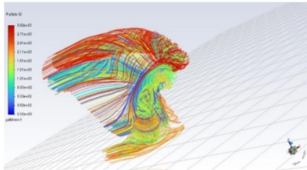
Gambar 13. Streamline FPP \phi 70 2 pitch
