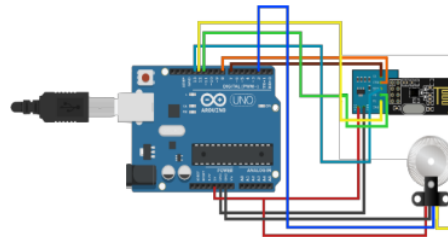
Gambar 4 Wiring Transmitter
