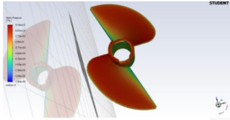
Gambar 5. Contour Pressure FPP ø40 2 pitch
