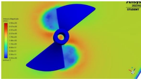
Gambar 12. Contour Velocity FPP \phi 70 2 pitch
