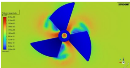
Gambar 15. Contour Velocity FPP \phi 70 3 pitch
