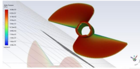
Gambar 8. Contour Pressure FPP ø45 2 pitch
