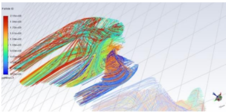
Gambar 10. Streamline FPP ø45 2 pitch
