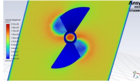
Gambar 9. Contour Velocity FPP ø45 2 pitch
