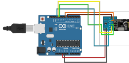
Gambar 3. Wiring Receiver
