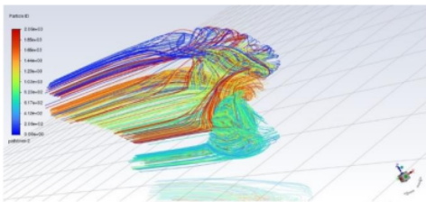
Gambar 7. Streamline FPP ø40 2 pitch
