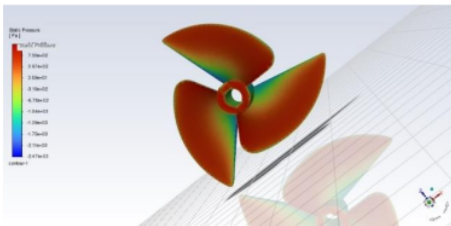
Gambar 14. Contour Pressure FPP \phi 70 3 pitch
