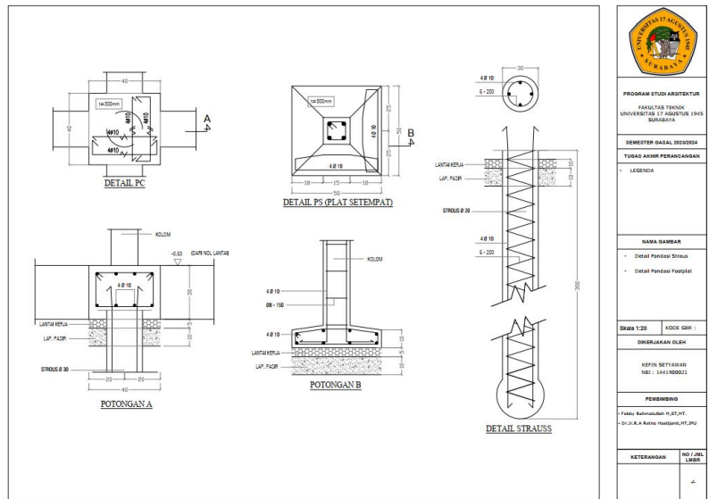
Gambar 6.4.14 Detail Pondasi
