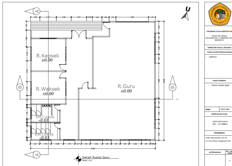
Gambar 6.2.14 Denah Ruang Guru
