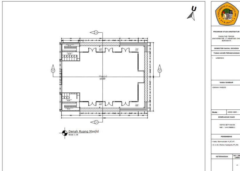
Gambar 6.2.10 Denah Masjid
