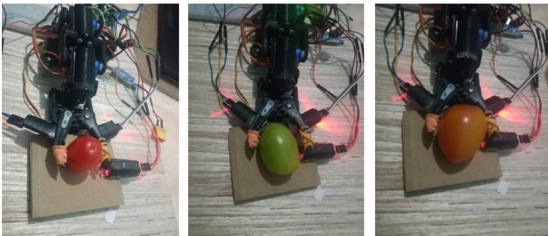
Gambar 6. Testing Robot
