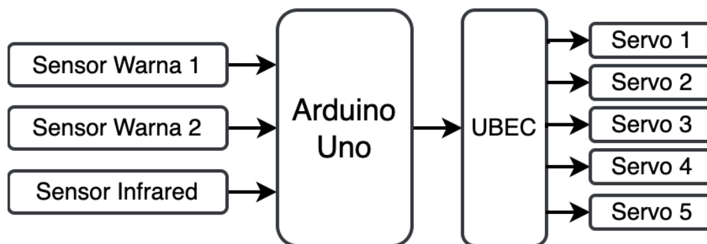
Gambar 1. Blok Diagram
