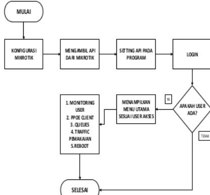
Gambar 2. Flowchart Website
